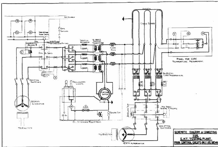
Figure 2—Diagram of Connections
