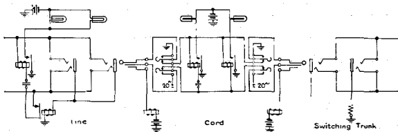
Figure 3—Schematic: Toll Switchboard No. 1 Circuits
