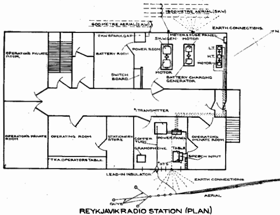
Figure 6—Reykjavik Radio Station—Plan of Main Floor
