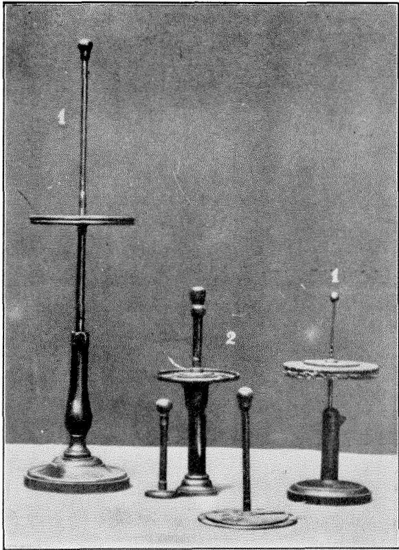
Figure 5—Volta's Condensing Electrostatic Machine (1). The condenser (2) is said to have been charged by the evaporation of liquids. These are from the Istituto Lombardo
