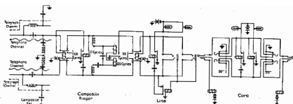
Figure 5—Schematic: Composite Ringer and Compositing Toll Line for Toll Switchboard No. 1
