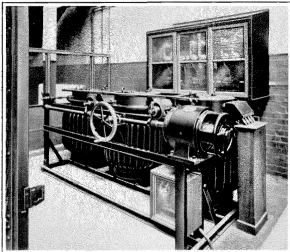
Figure 6—Induction Regulators
