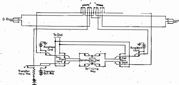
Figure 7—Schematic: Toll Cord Positional Circuit; talking key operated for toll switchboard No. 3
