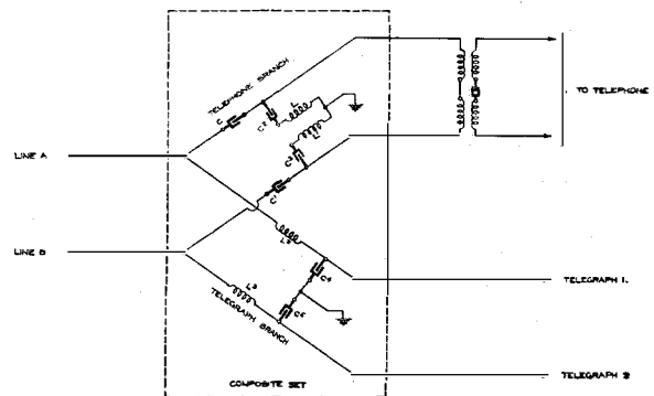
Figure 1—Schematic of Composite Set
